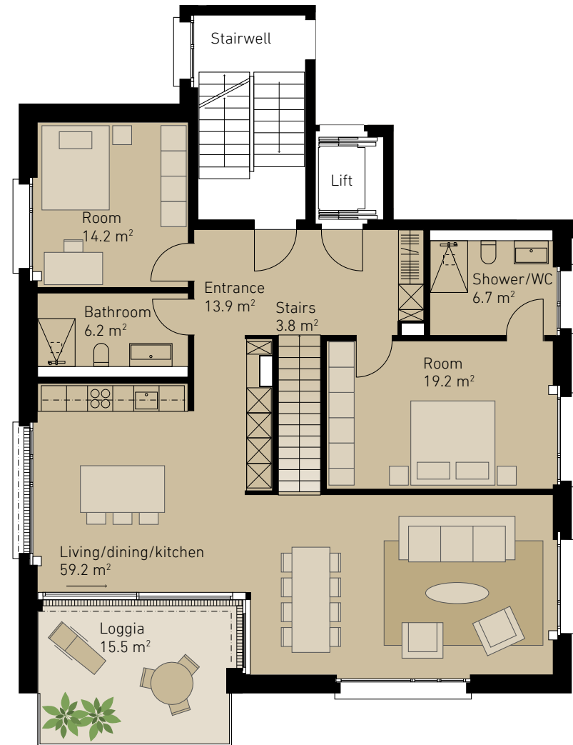
1 st floor
